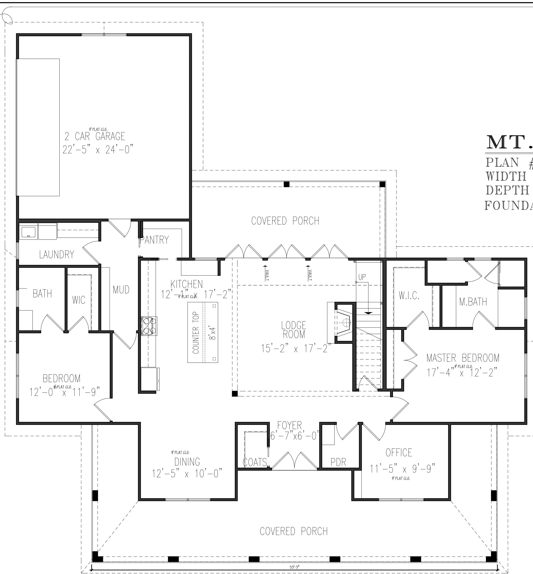
1st FLOOR PLAN 2,970 SQ. FT.
