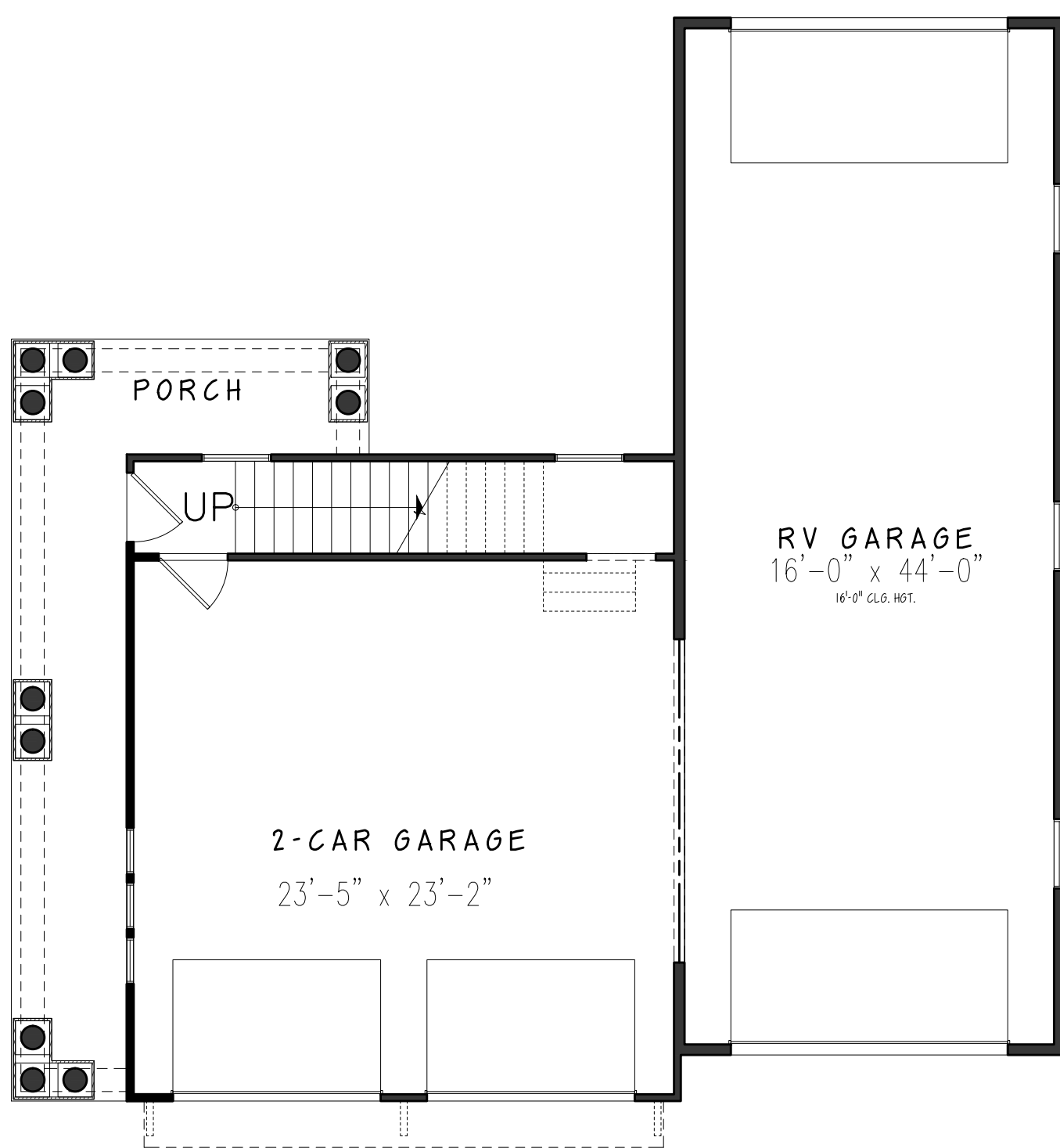
2-CAR GARAGE 573 SQ. FT. RV GARAGE 750 SQ. FT.
