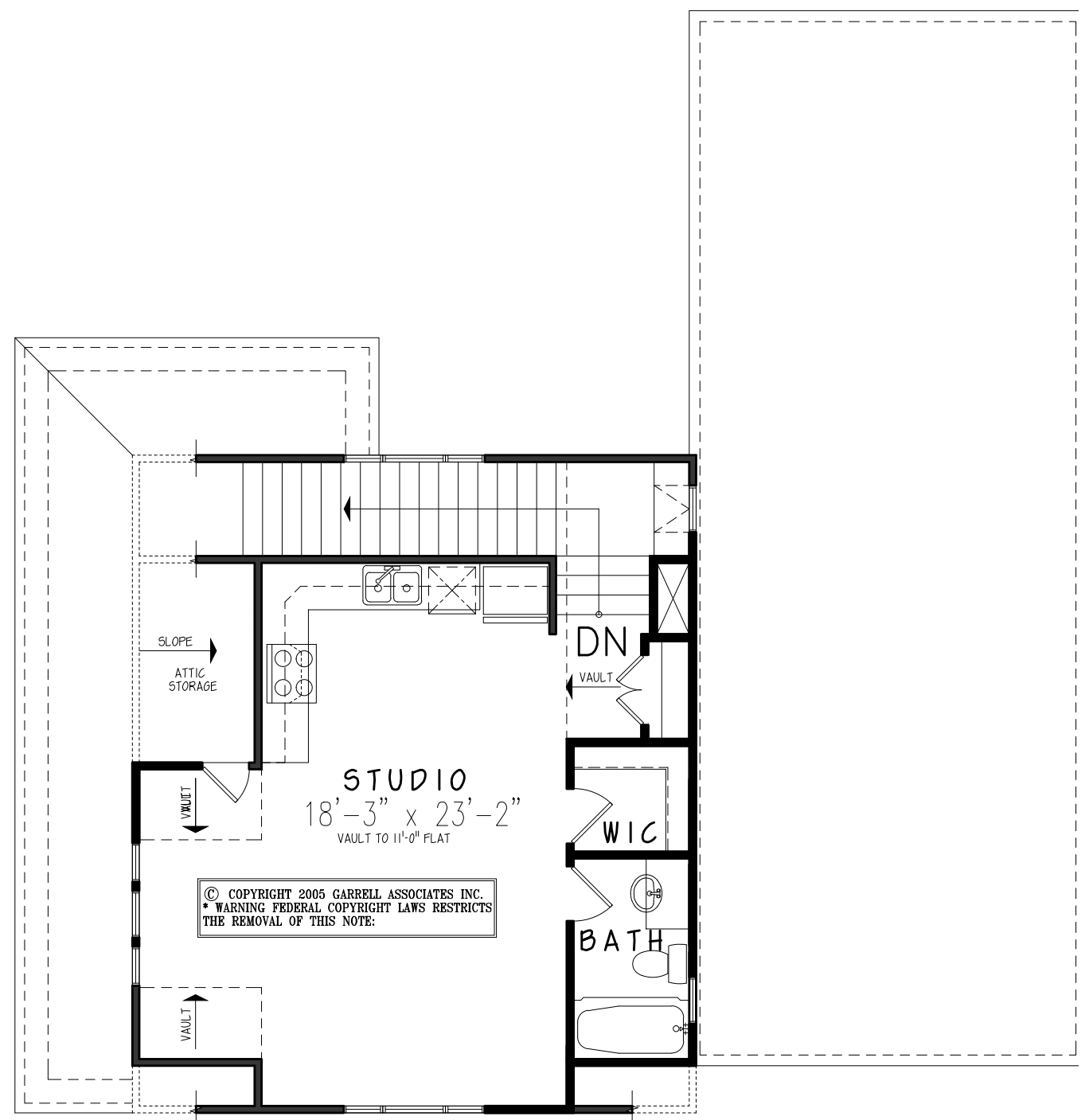
SECOND FLOOR PLAN 651 SQ.FT. STORAGE 42 SQ.FT.
