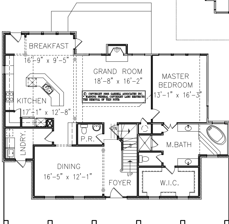
1st FLOOR PLAN 1733 SQ. FT.
