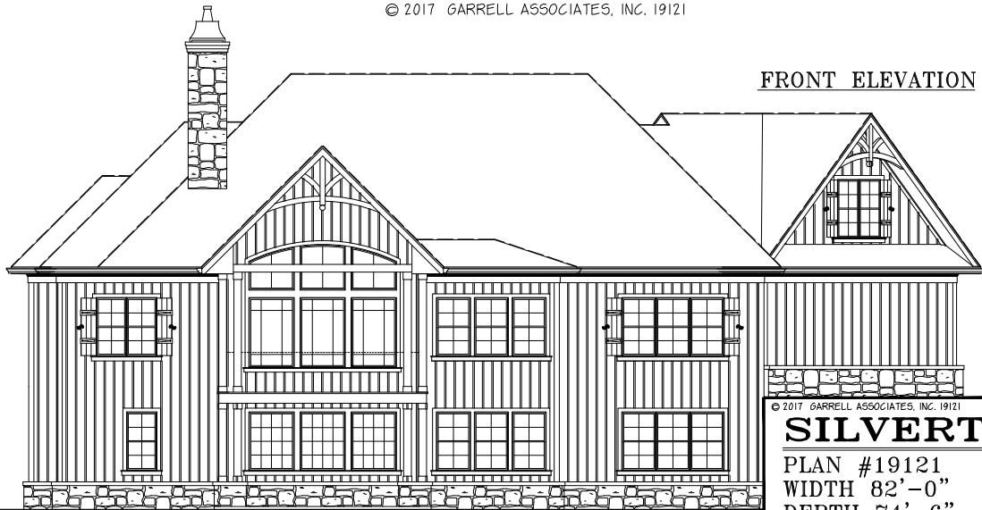
REAR ELEVATION
