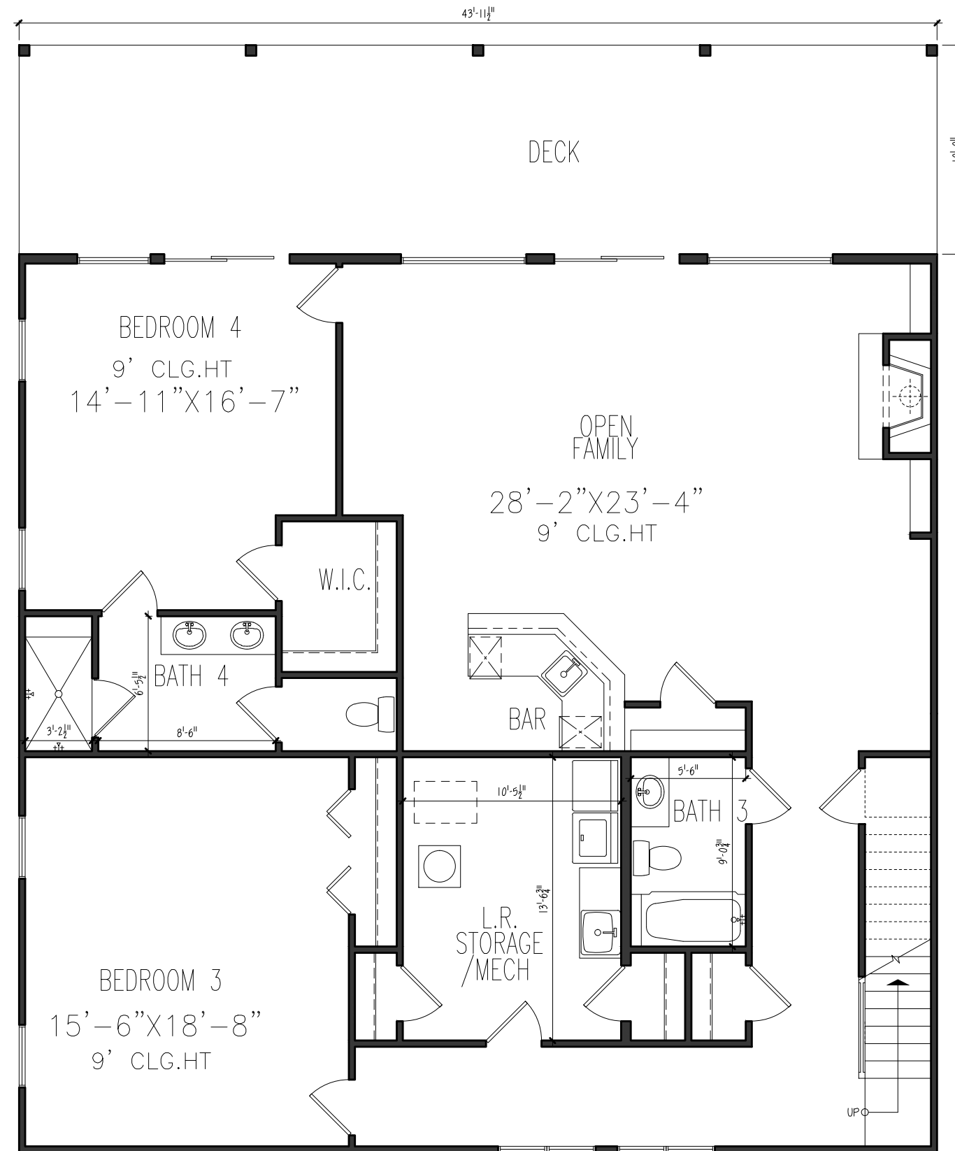
BASEMENT PLAN 1696 SQ.FT.
