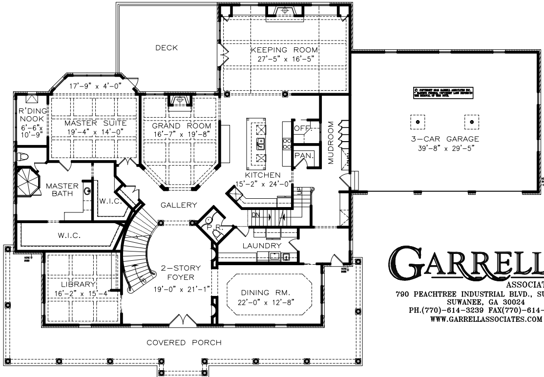
1st FLOOR PLAN 3,940 SQ. FT. GARAGE 1,200 SQ. FT.
