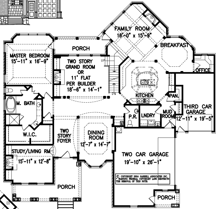
1st FLOOR PLAN 2491 SQ. FT. GARAGE 746 SQ. FT.
