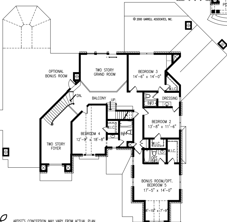
SECOND FLOOR PLAN 1,278 SQ.FT. OPT.B. RM.#5 428 SQ.FT.
