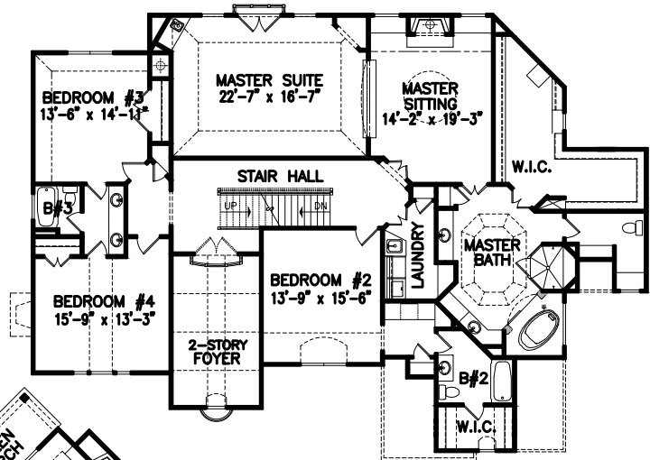
2nd FLOOR PLAN 2494 SQ. FT.
