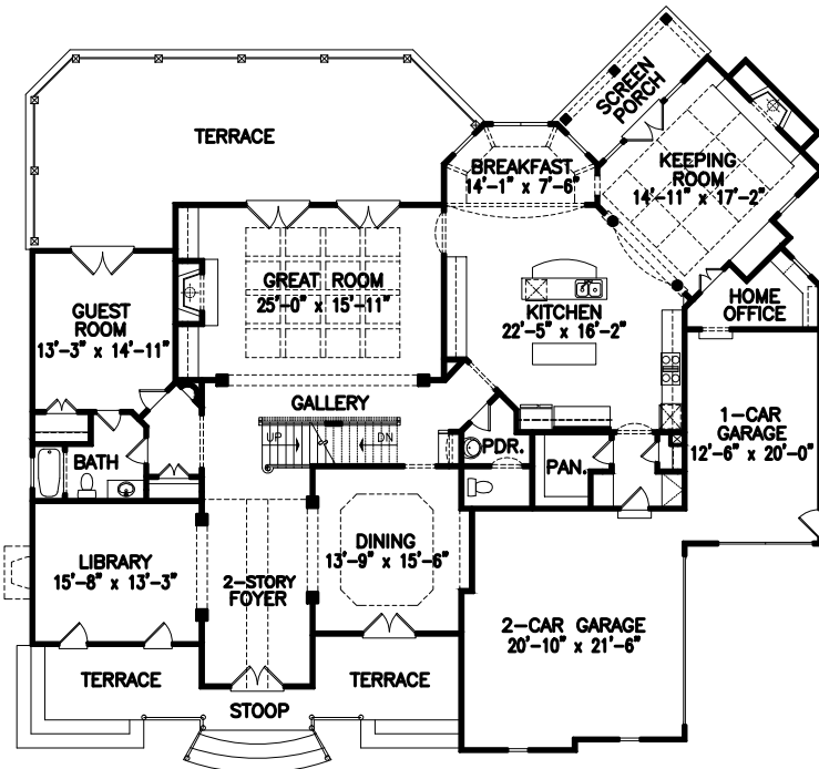
1st FLOOR PLAN 2701 SQ. FT. GARAGE 724 SQ. FT.
