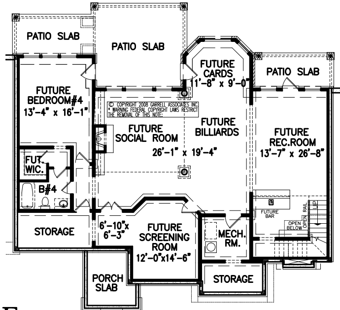
OPT. BSMT. PLAN 1711 SQ. FT.
