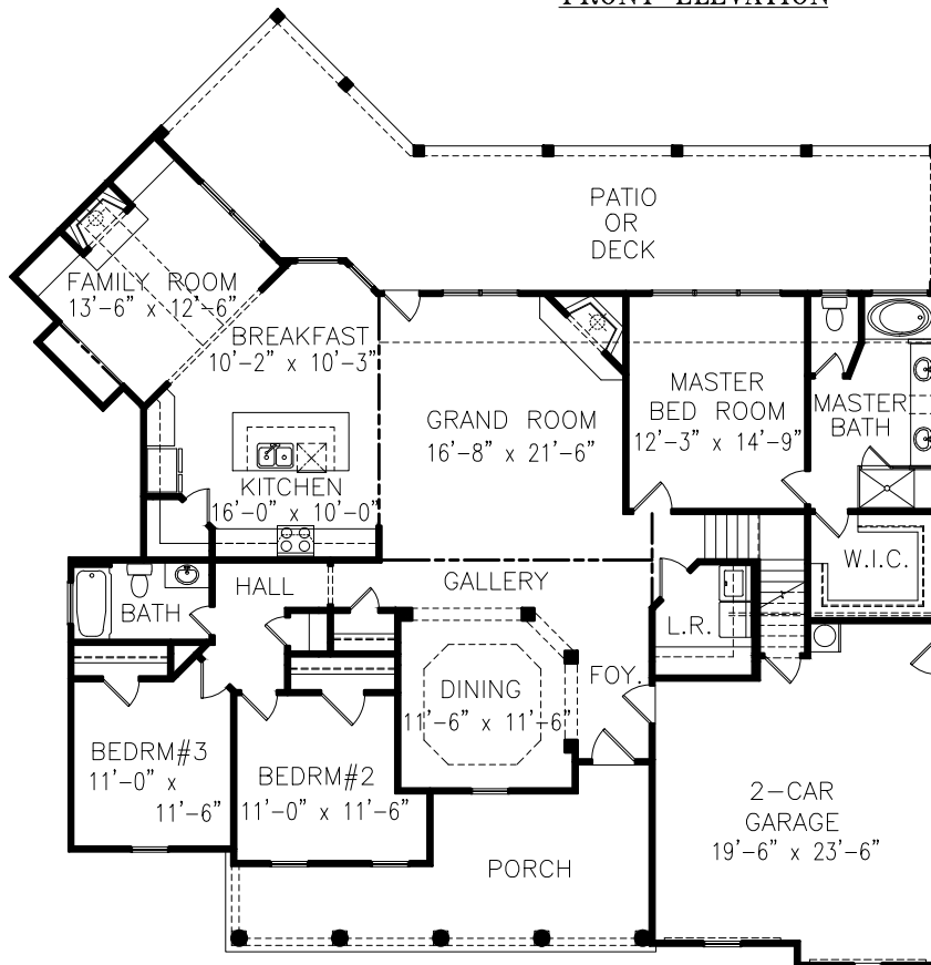
1st FLOOR PLAN 2061 SQ. FT.
