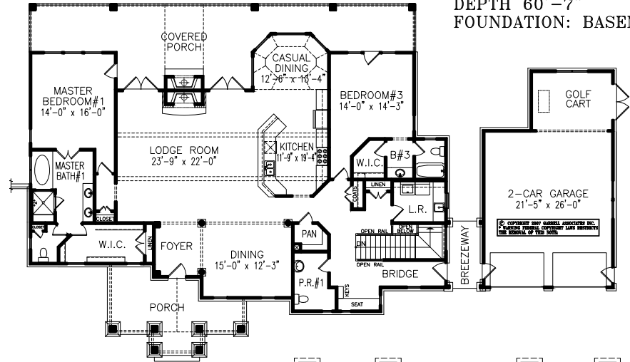
1st FLOOR PLAN 2580 SQ. FT. GARAGE 725 SQ. FT.
