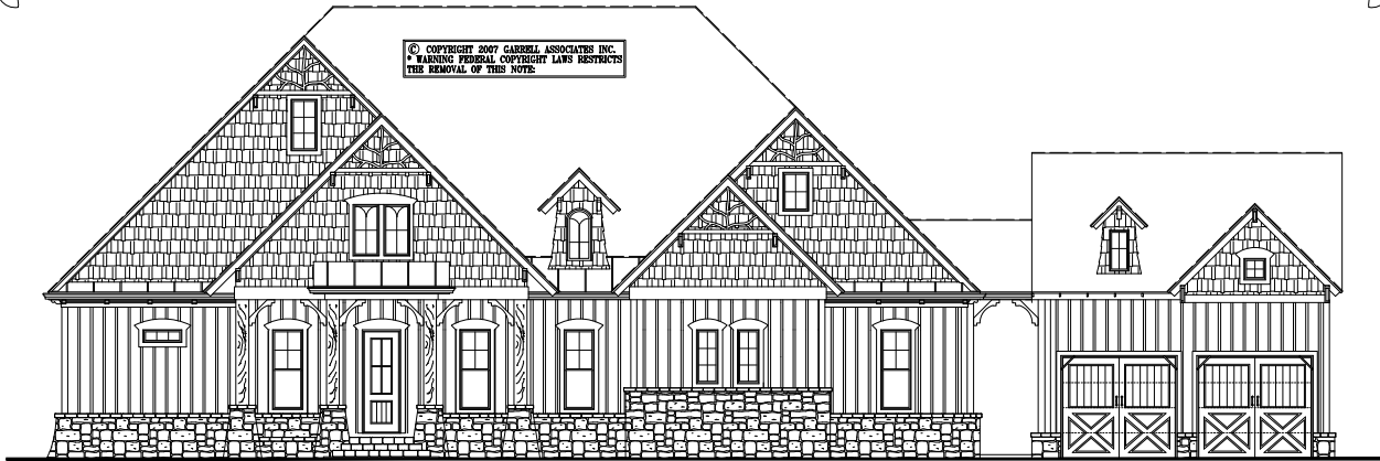
FRONT ELEVATION
