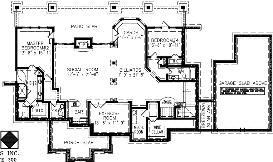
TERRACE LEVEL 2361 SQ. FT.
