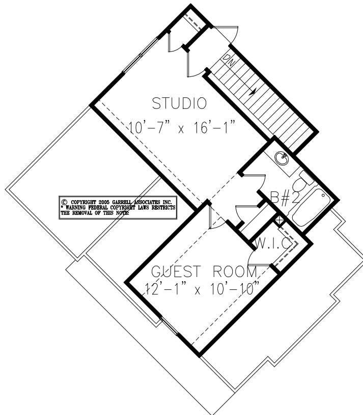
2nd FLOOR PLAN 458 SQ. FT.
