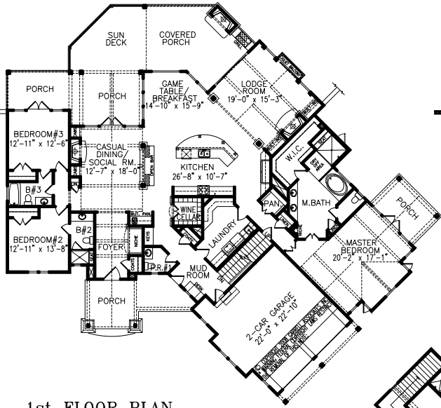
1st FLOOR PLAN 3070 SQ. FT. GARAGE 552 SQ. FT.
