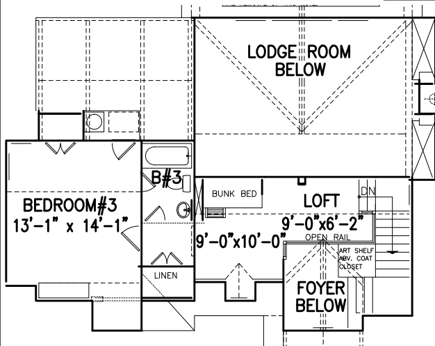
2nd FLOOR PLAN 490 SQ. FT.
