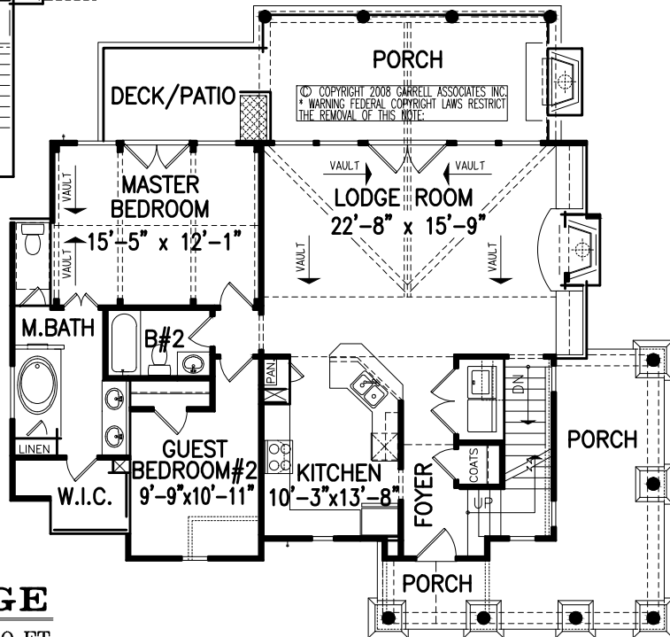
1st FLOOR PLAN 1264 SQ. FT.
