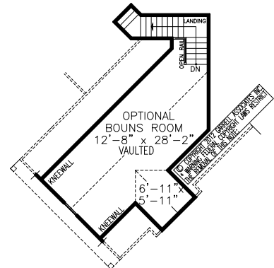
OPT. 2nd FLOOR PLAN 426 SQ. FT.
