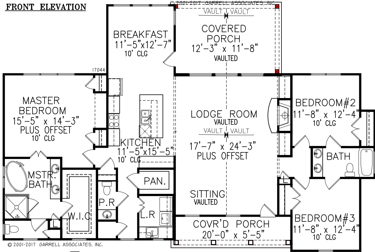
1st FLOOR PLAN 1,925 SQ. FT.
