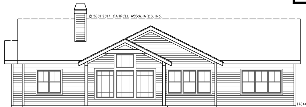
REAR ELEVATION
