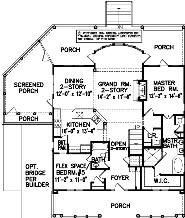
1st FLOOR PLAN 1612 SQ. FT.
