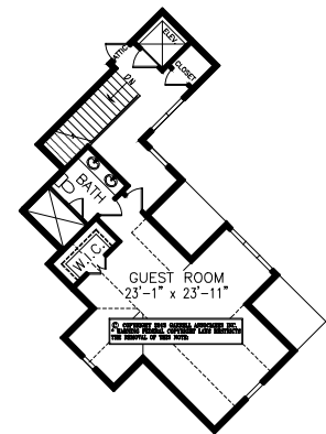
2nd FLOOR PLAN 699 SQ.FT.
