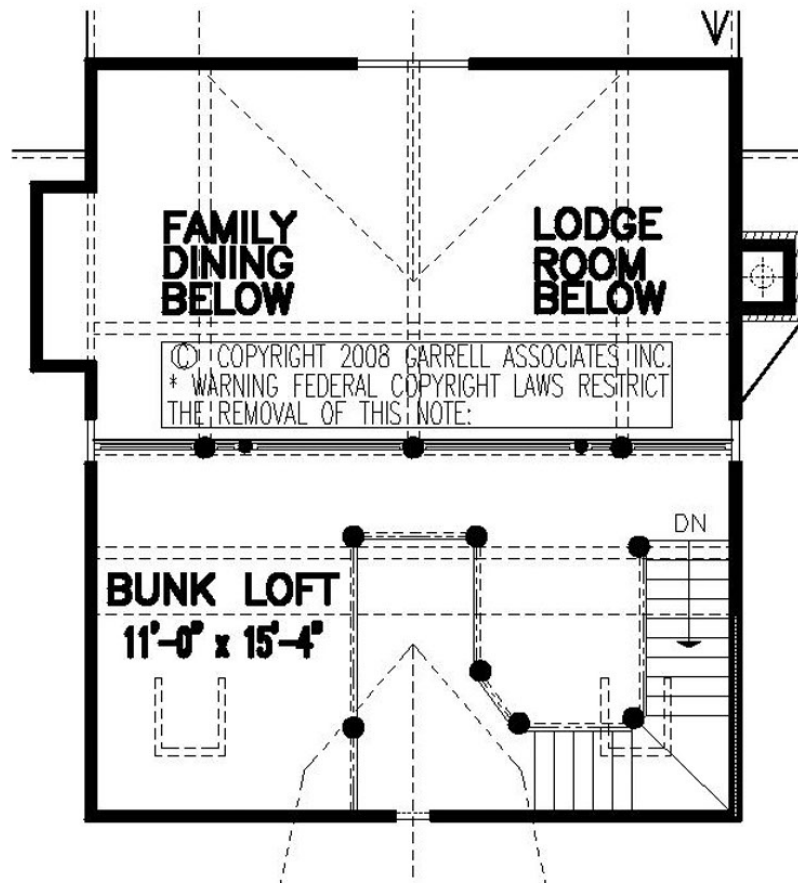
OPTIONAL LOFT PLAN ADDITIONAL 386 SQ. FT.
