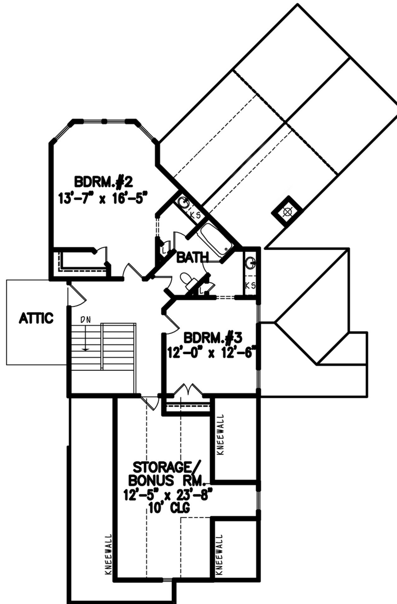
SECOND FLOOR PLAN 728 SQ. FT.
