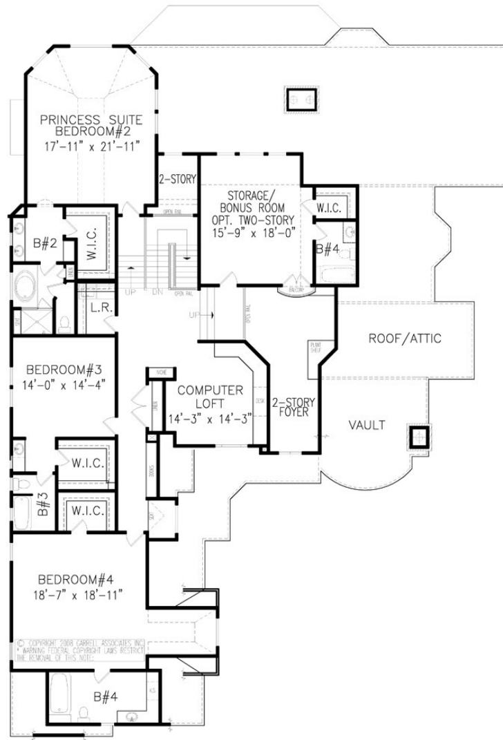
SECOND FLOOR PLAN 2,204 SQ. FT.
