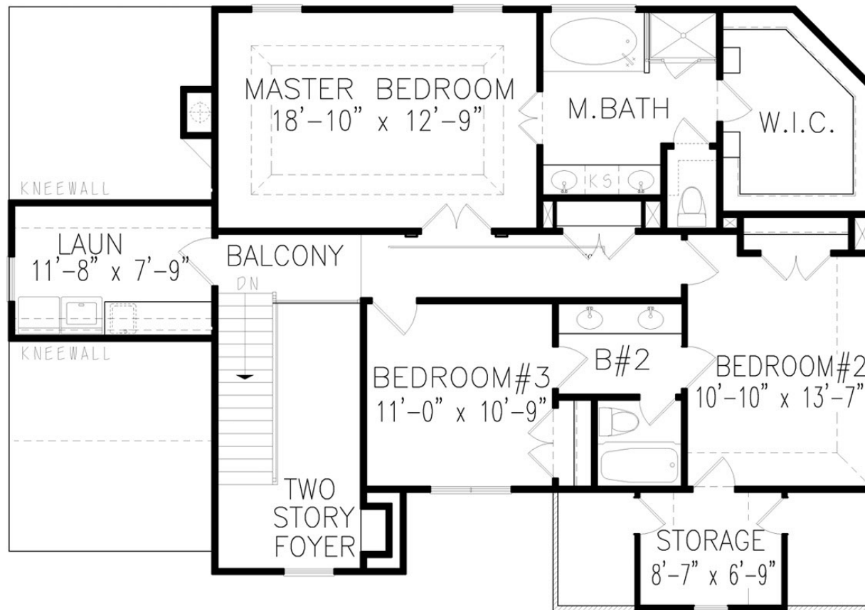
SECOND FLOOR PLAN 1,052 SQ. FT.
