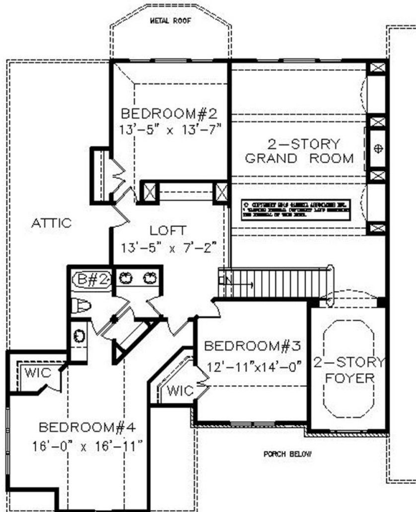
2nd FLOOR PLAN 1,017 SQ. FT.
