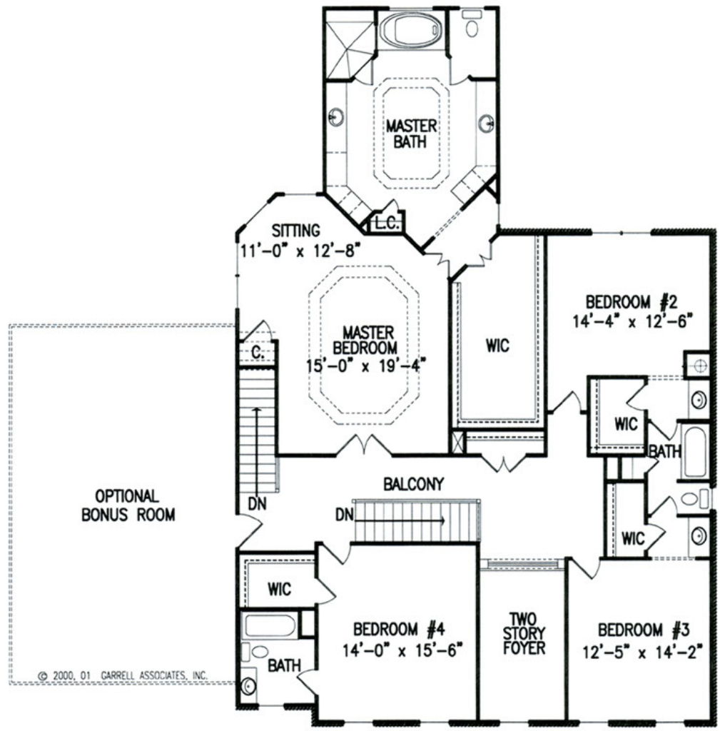
SECOND FLOOR PLAN 2,147 SQ. FT.
