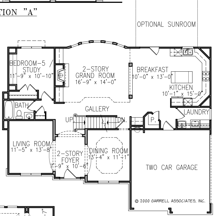
FIRST FLOOR PLAN 1,555 SQ.FT. GARAGE 449 SQ.FT.
