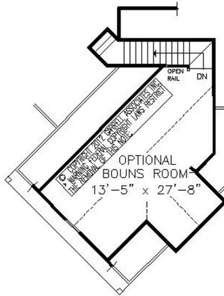
OPT. 2nd FLOOR PLAN 428 SQ. FT.
