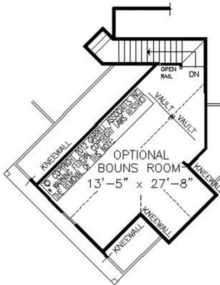
OPT. 2nd FLOOR PLAN 428 SQ. FT.
