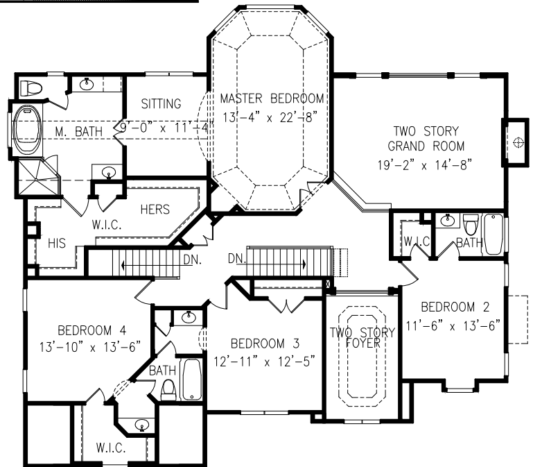
SECOND FLOOR PLAN 1,699 SQ. FT.
