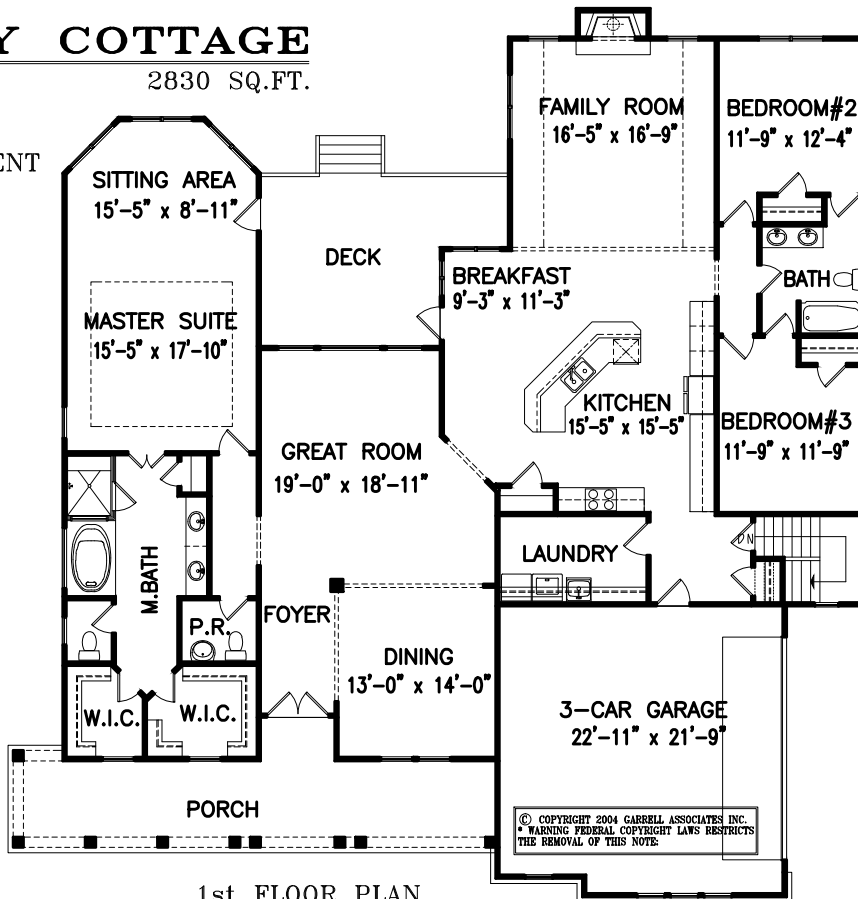
1st FLOOR PLAN 2830 SQ. FT. GARAGE 684 SQ. FT.
